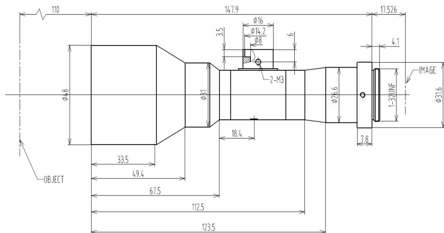
SMT11IR075W110C-L
