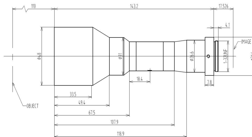
SMT11IR075W110C-I
