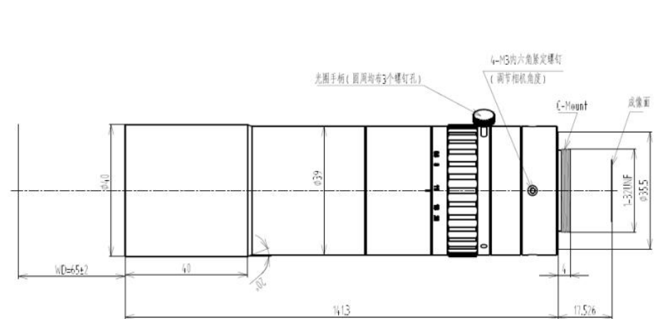
SMT11IR075W65C-I
