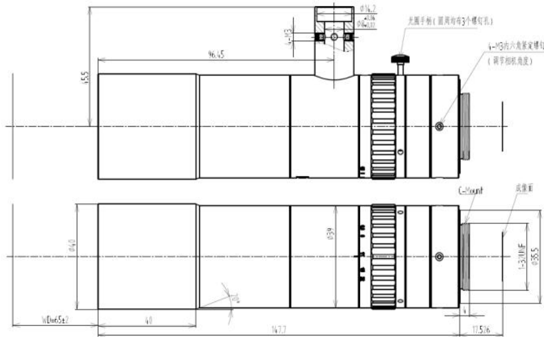
SMT11IR075W65C-L
